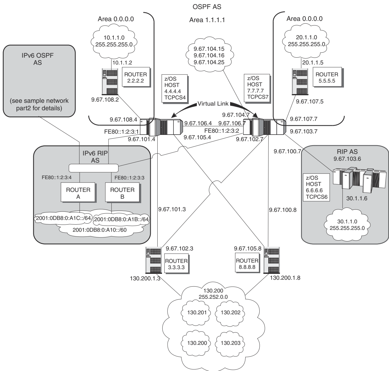
Figure 48. Sample network part 1
