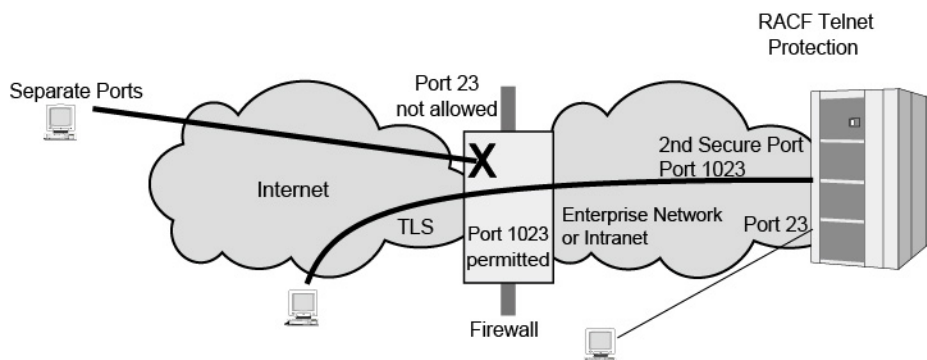
Figure 34. Using multiple Telnet ports to separate secure and non-secure traffic
