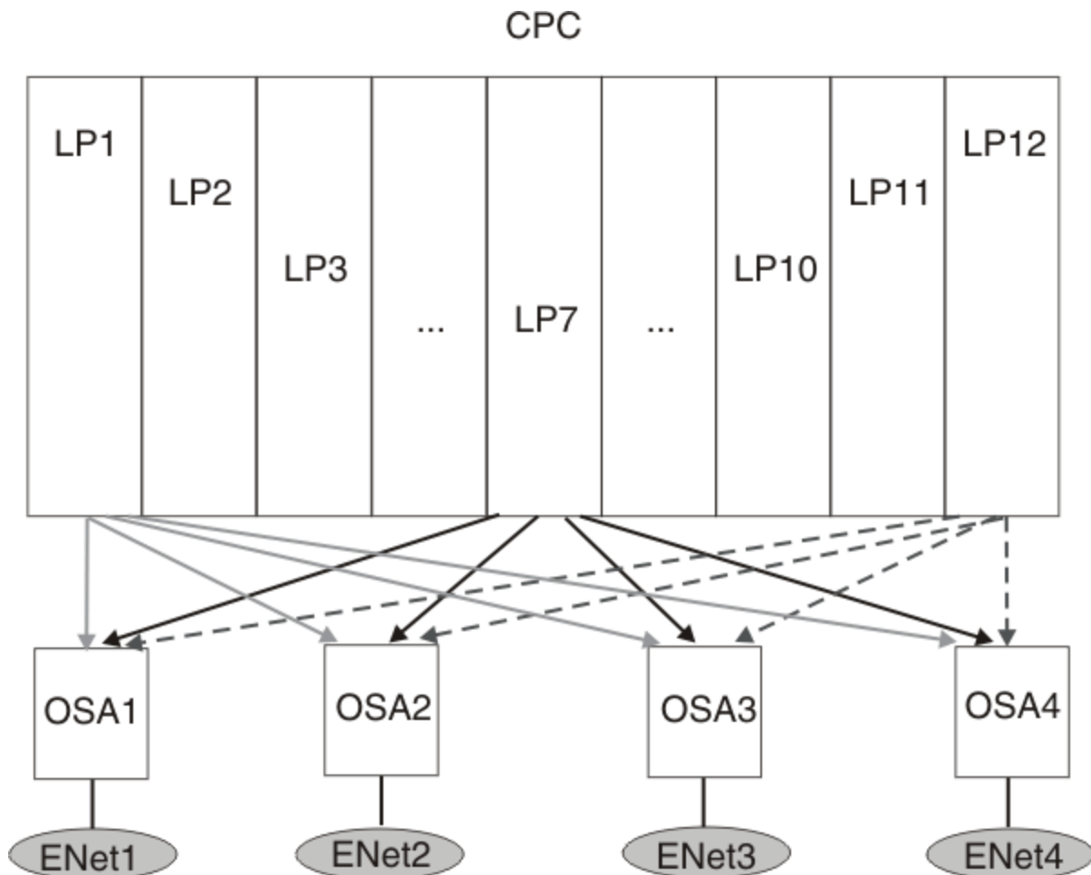
Figure 17. Candidate configuration for HiperSockets Accelerator
