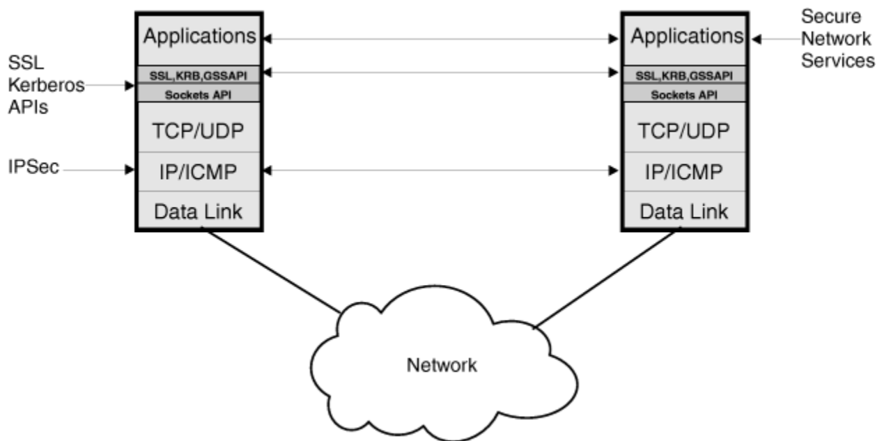
Figure 31. Security protocols from a protocol layering perspective
