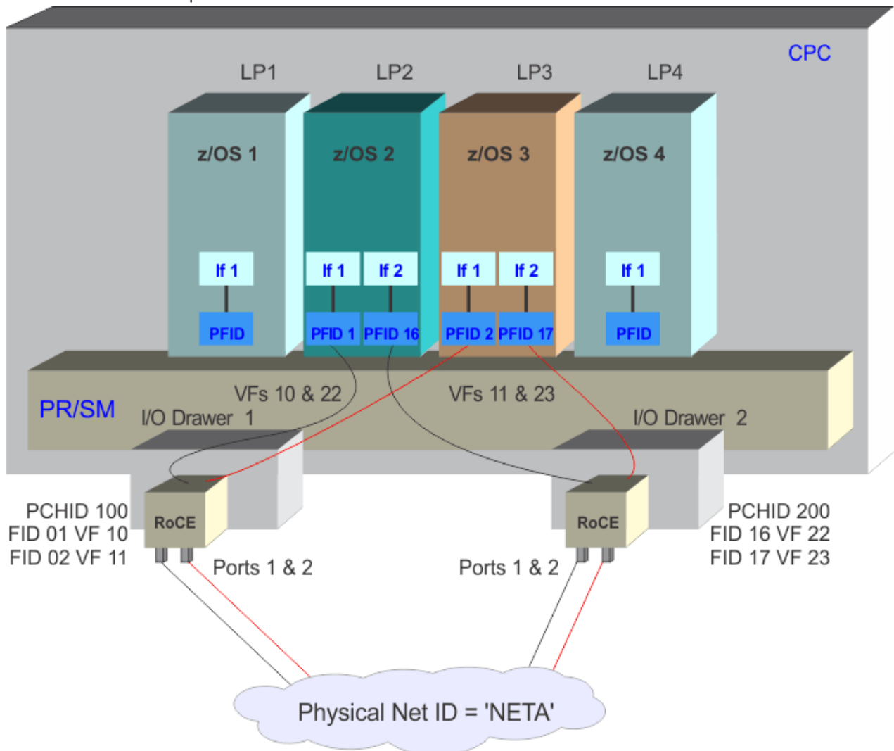
Figure 65. 10 GbE RoCE Express feature in a shared RoCE environment
