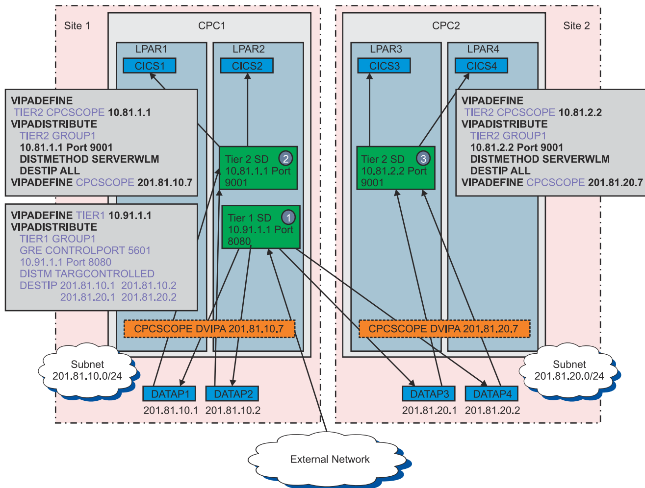
Figure 61. Sysplex distributor load balancing to DataPower in a multi-tier and multisite environment
