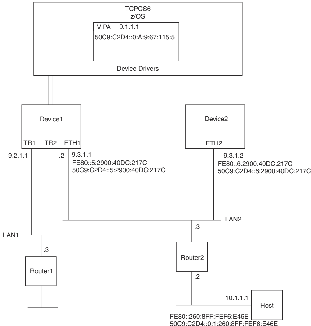
Figure 50. Static VIPA configuration
