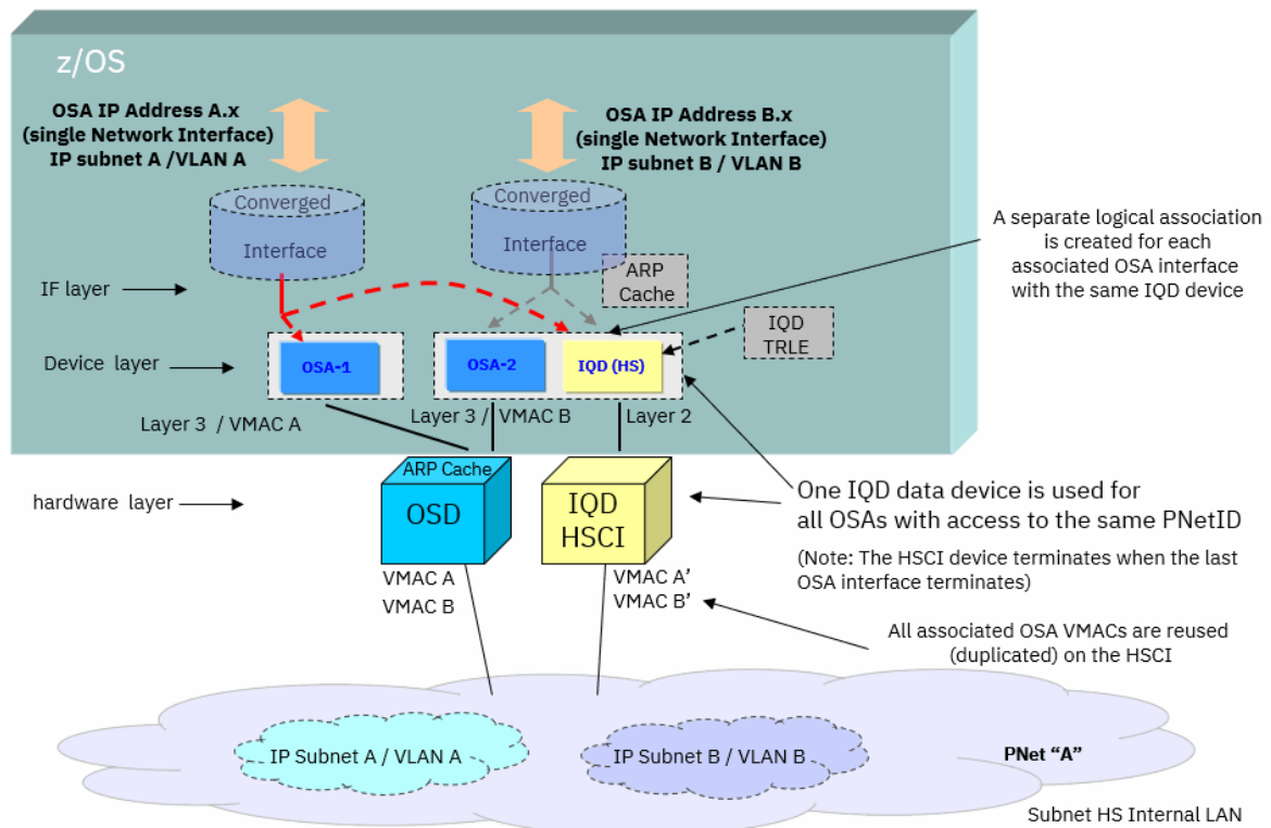
Figure 23. An HSCI sample configuration with a single OSA-Express feature, two IP interfaces and two subnets
