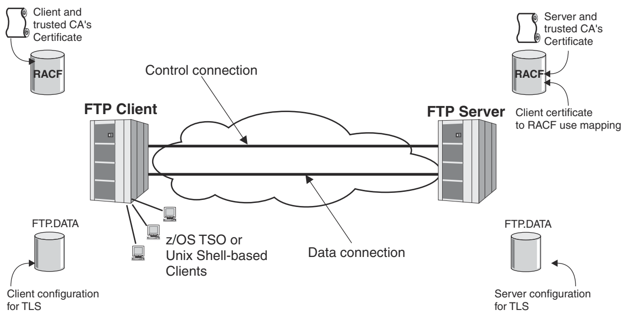
Figure 37. FTP client and server TLS overview
