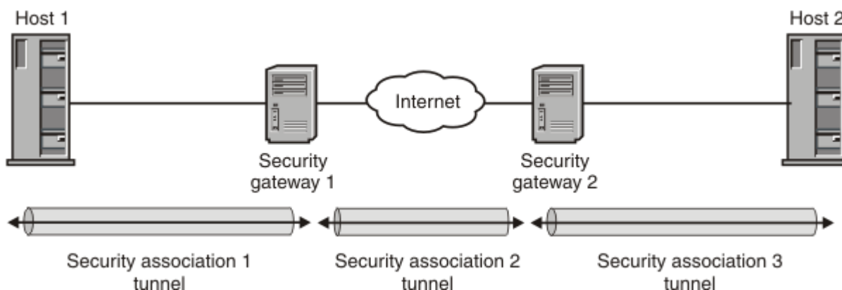
Figure 126. Cascaded tunnels
