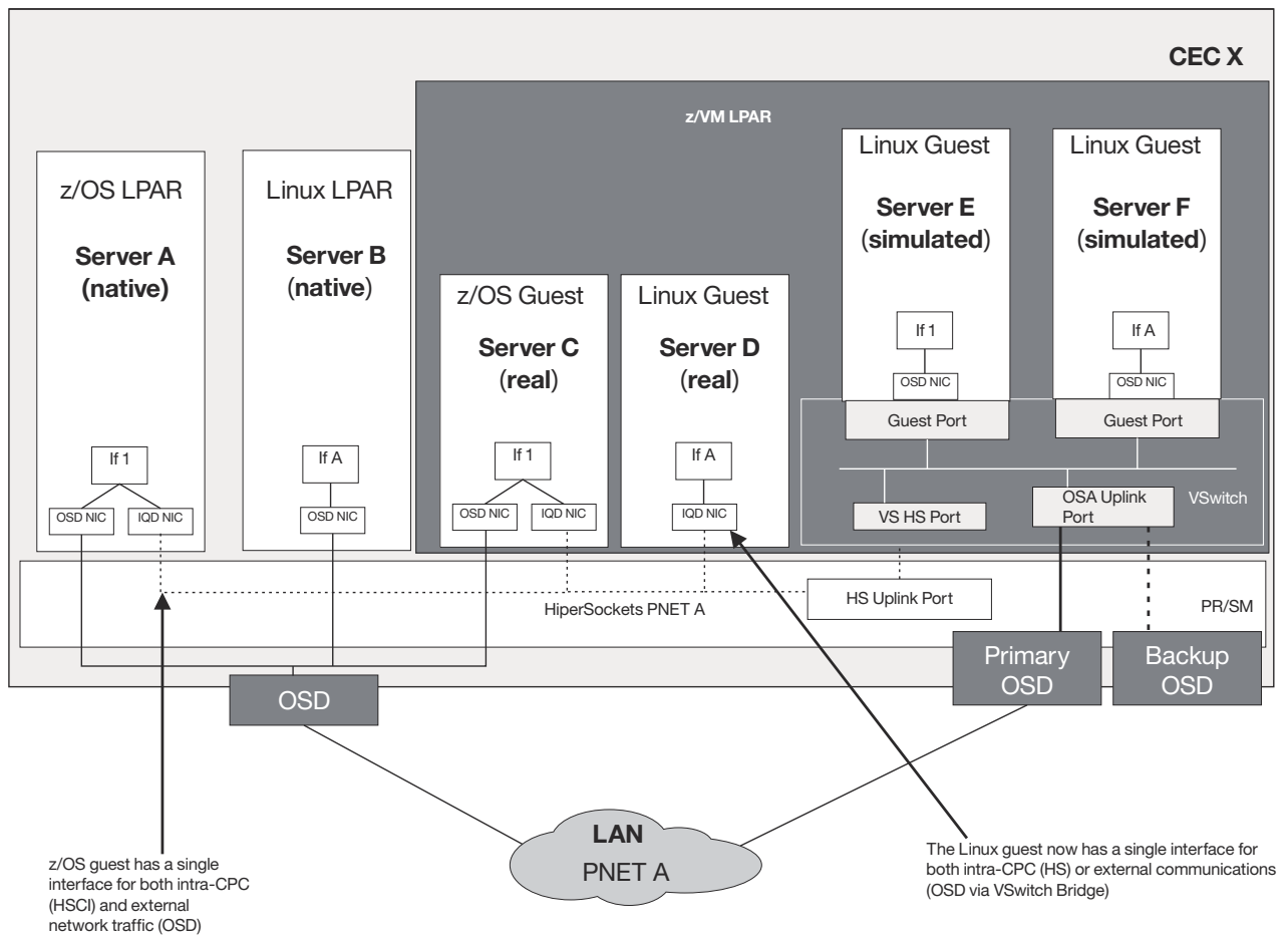
Figure 24. Linux and z/VM VSwitch bridge environment
