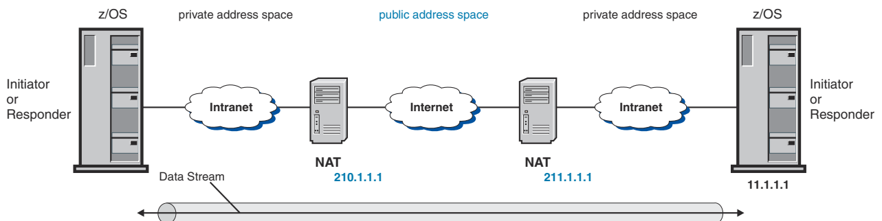
Figure 128. z/OS host to z/OS host, double NAT
