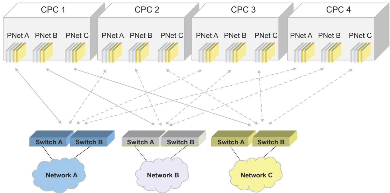
Figure 73. Physical networks
