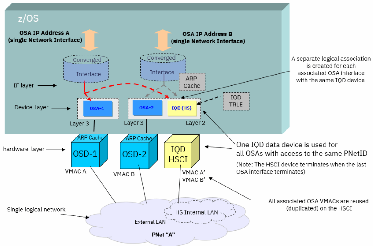
Figure 22. An HSCI sample configuration with two OSA-Express features, two IP interfaces and a single subnet
