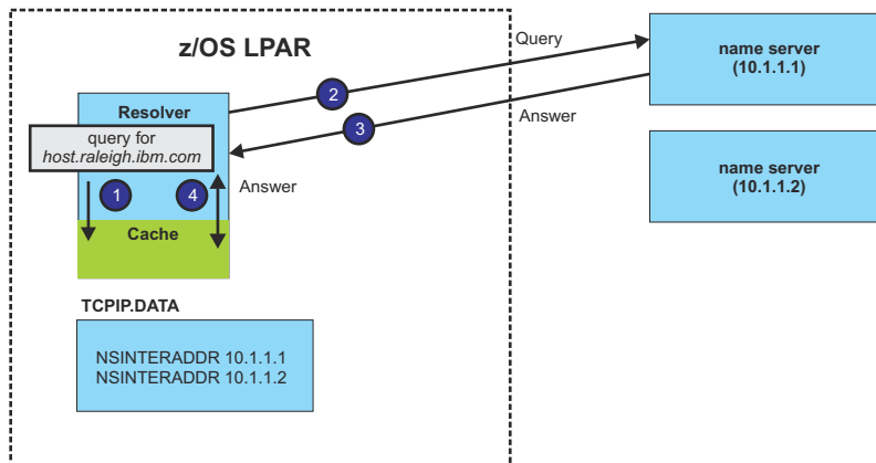
Figure 98. Resolver caching example
