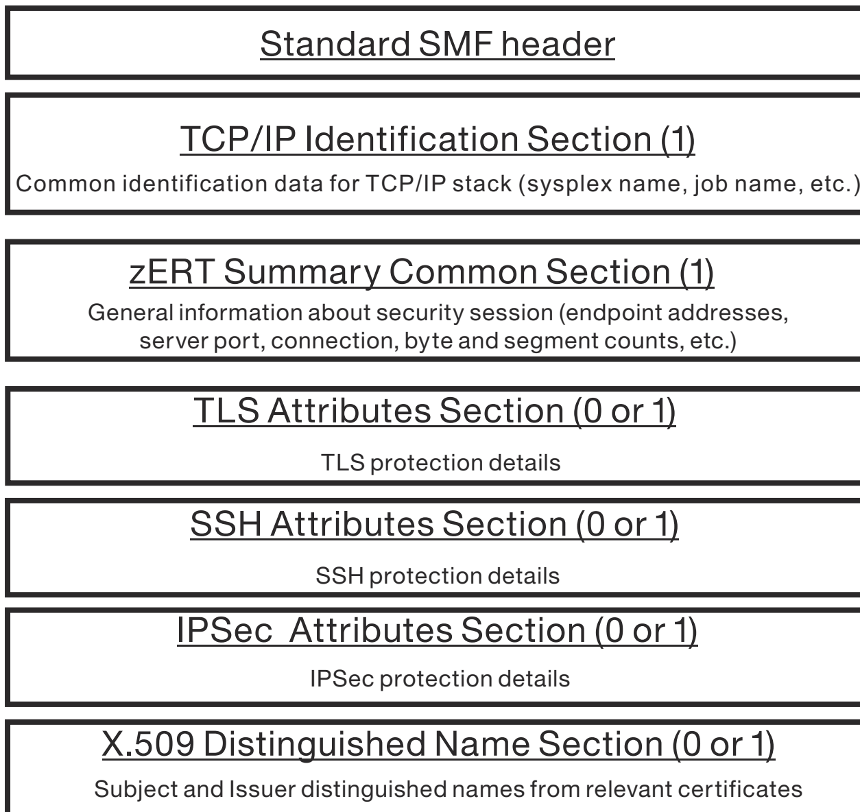
Figure 39. zERT summary (SMF 119 subtype 12) record layout
