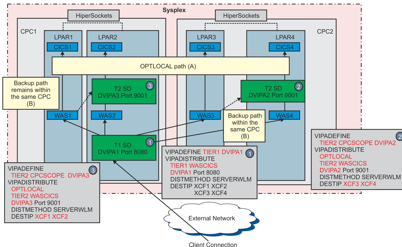
Figure 58. z/OS multi-tier application configuration using CPCSCOPE DVIPAs
