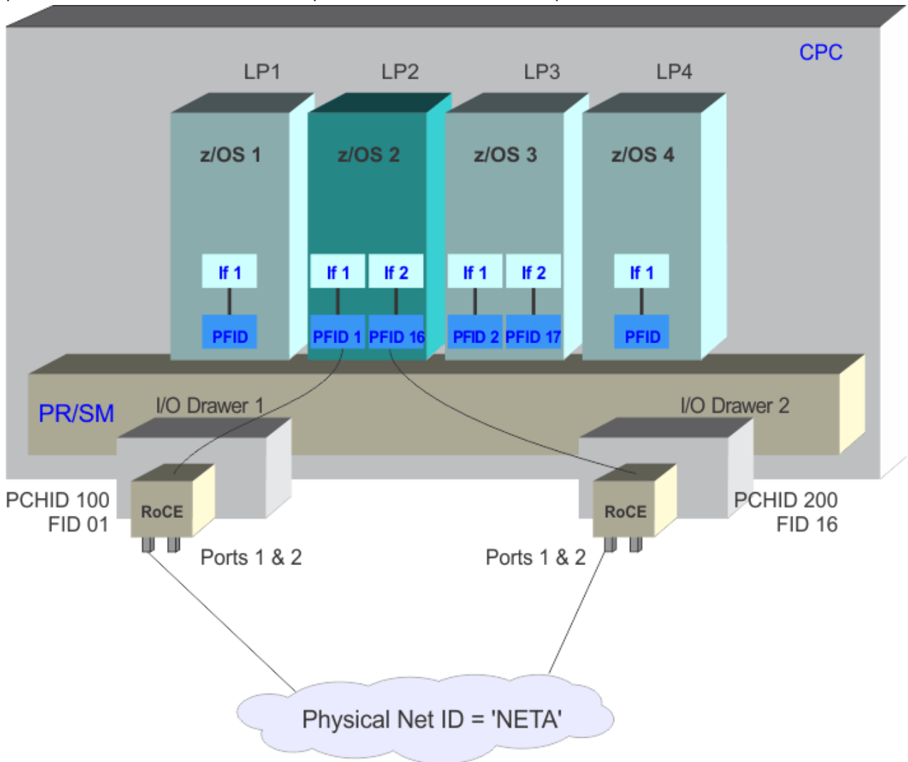
Figure 64. 10 GbE RoCE Express feature in a dedicated RoCE environment
