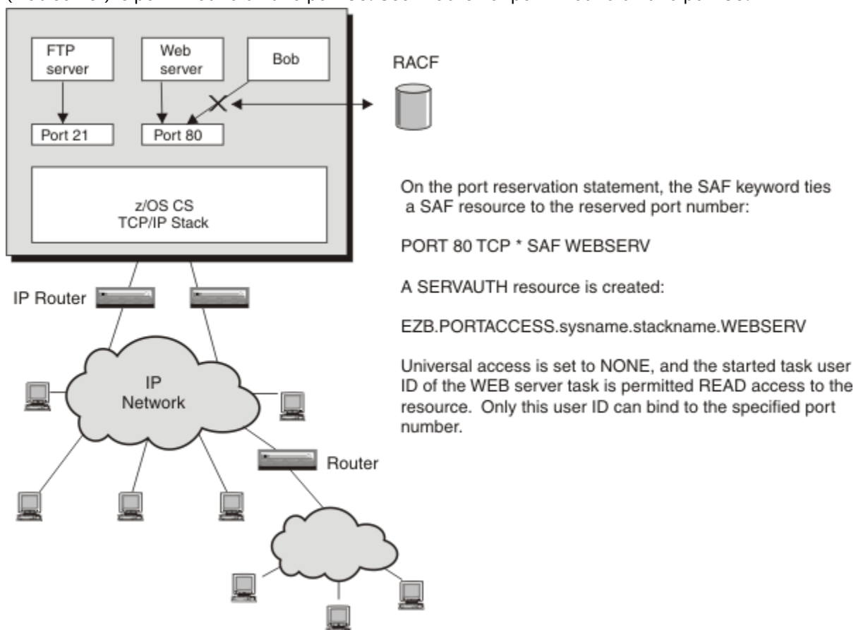
Figure 28. Port access control overview
