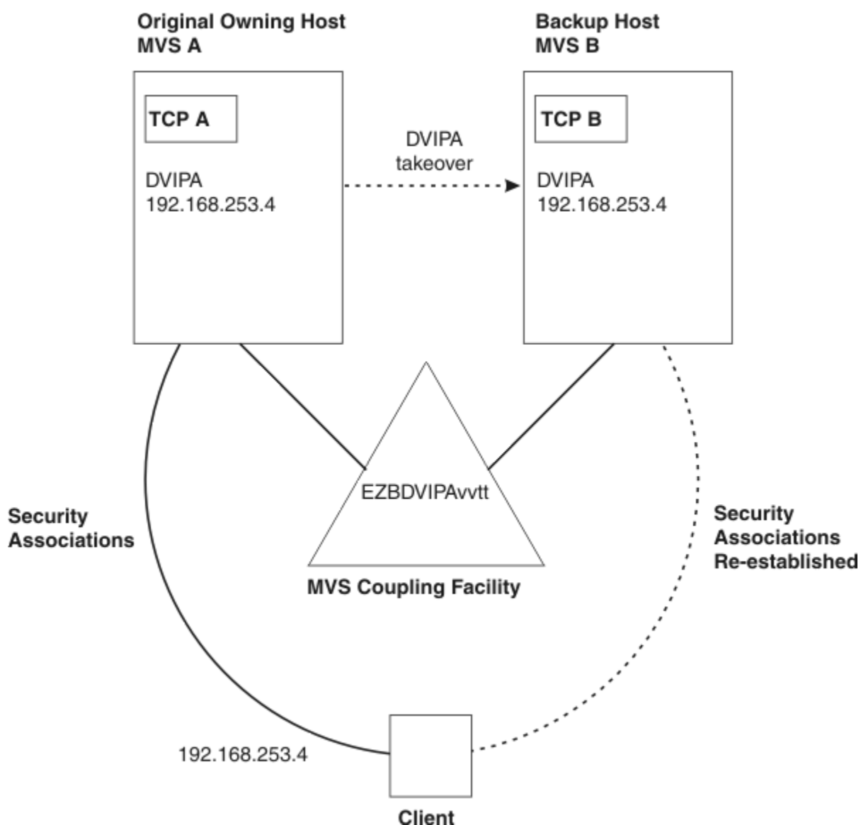
Figure 53. DVIPA takeover with SWSA
