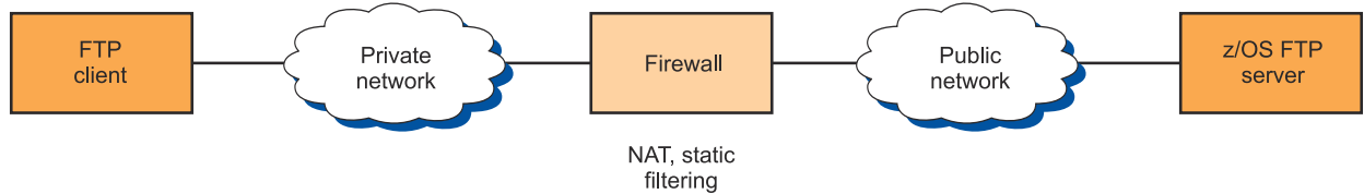
Figure 92. SSL/TLS-secured FTP session scenario 3
