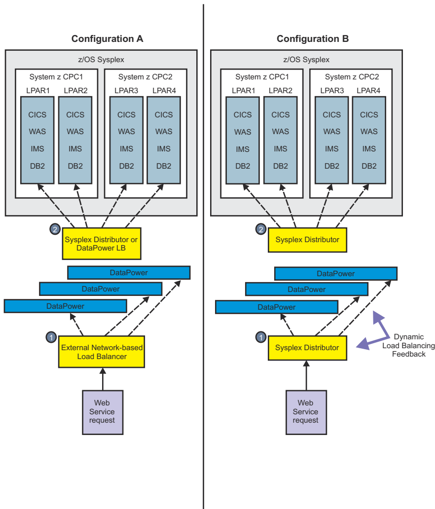
Figure 59. DataPower load balancing overview
