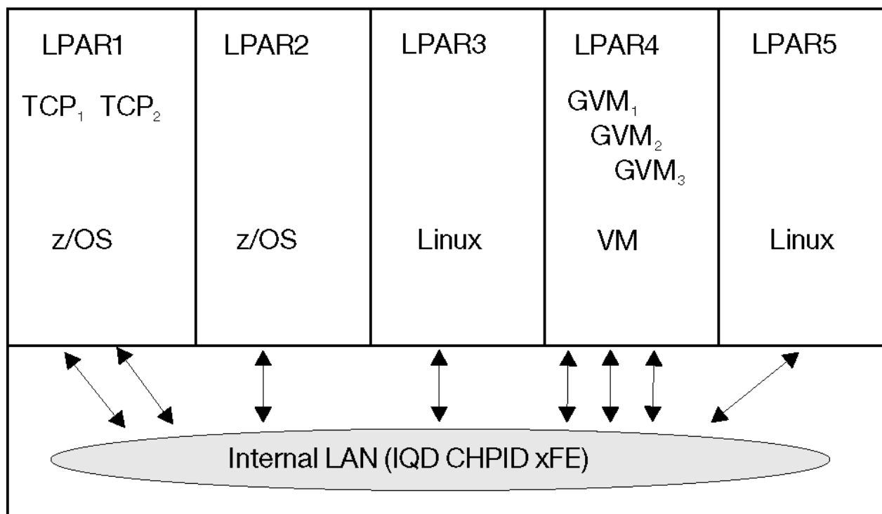
Figure 14. HiperSockets internal LAN
