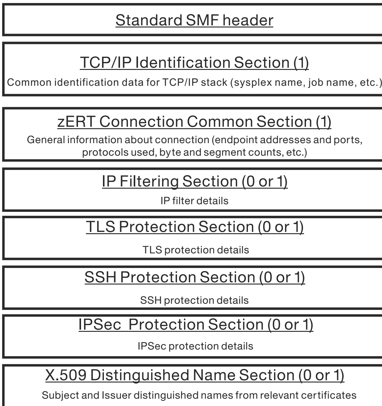
Figure 38. zERT connection detail (SMF 119 subtype 11) record layout
