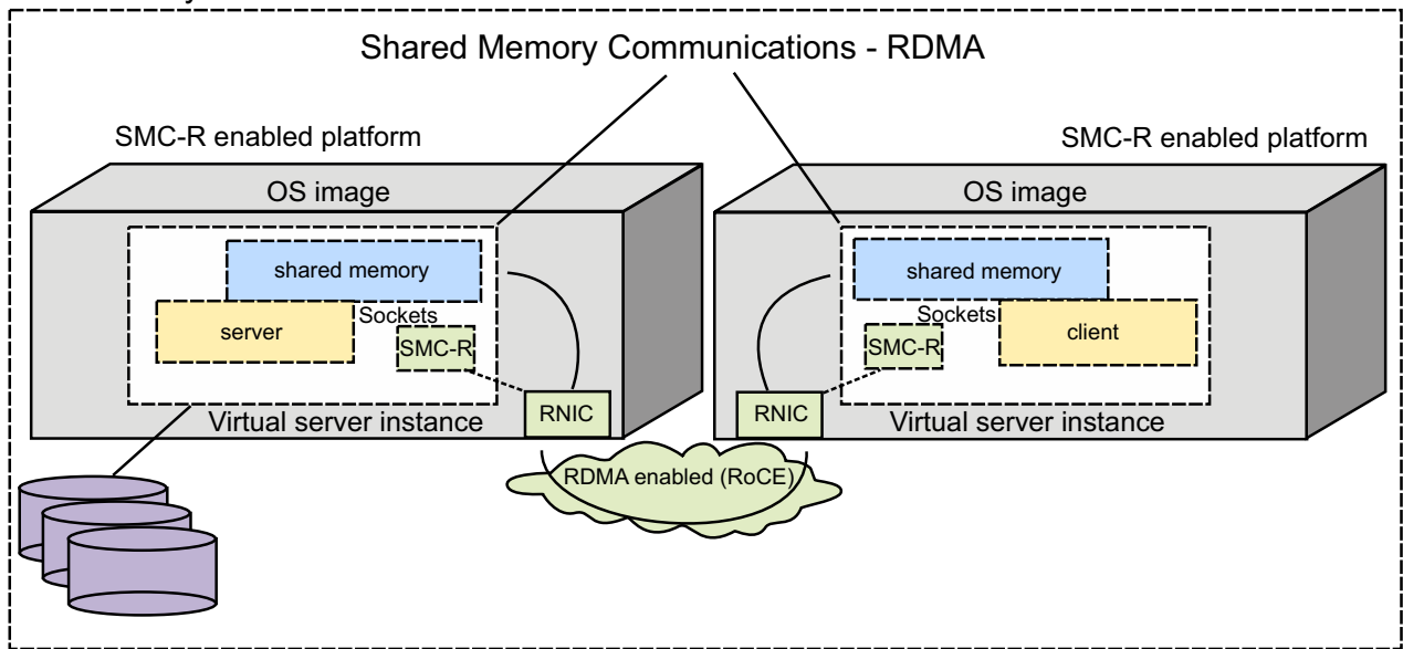
Figure 63. Shared Memory Communications over RDMA (SMC-R)
