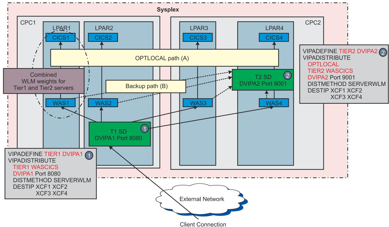
Figure 57. Enhanced z/OS multi-tier application load balancing using sysplex distributor
