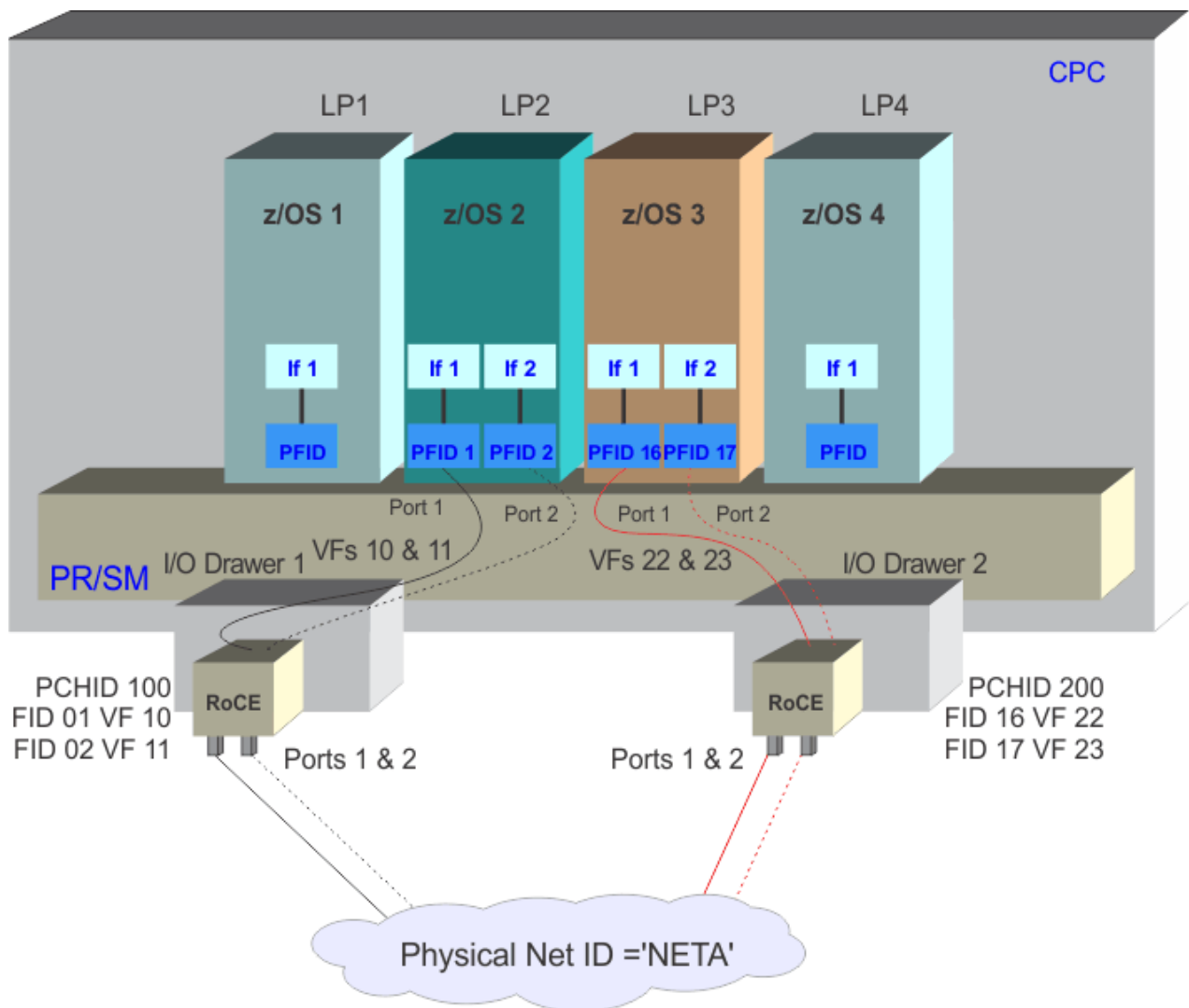
Figure 75. Misleading full redundancy configuration in a shared RoCE environment
