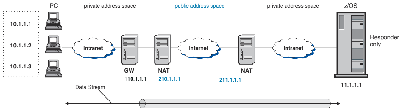
Figure 130. z/OS in a host-to-security gateway configuration
