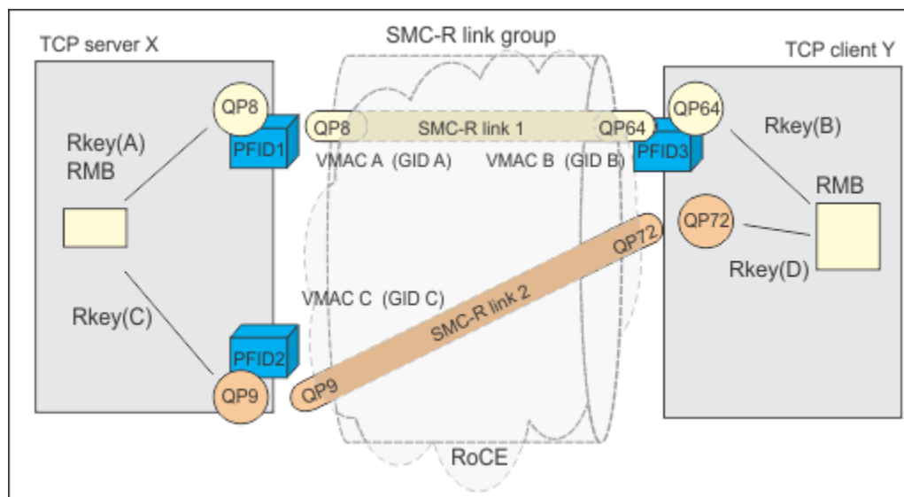
Figure 77. Partially redundant SMC-R links
