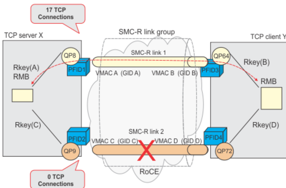
Figure 76. Failover processing within an SMC-R link group
