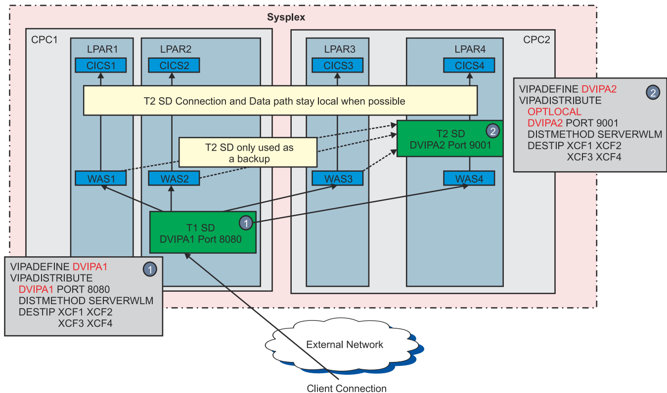
Figure 56. z/OS multi-tier application load balancing using sysplex distributor and the OPTLOCAL keyword
