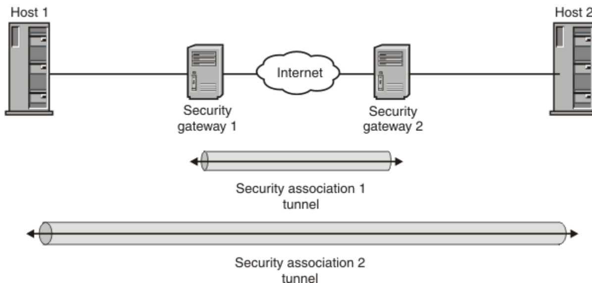
Figure 127. Nested tunnels
