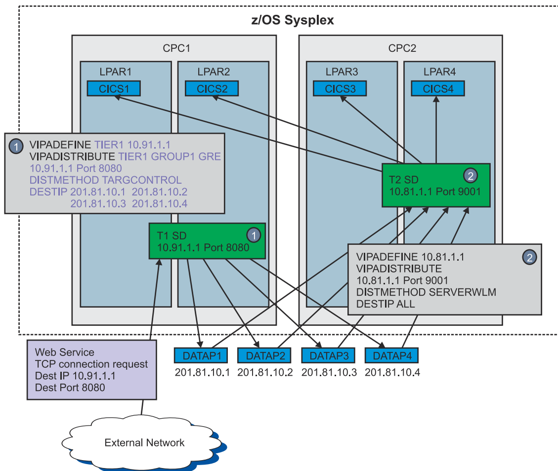
Figure 60. Sysplex distributor load balancing for DataPower
