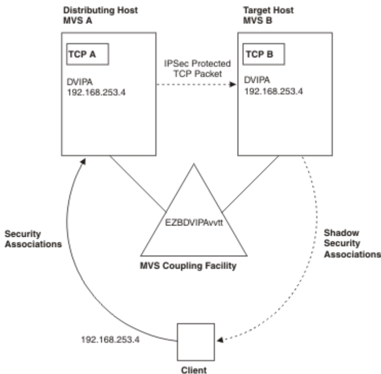
Figure 54. Sysplex distributor with SWSA
