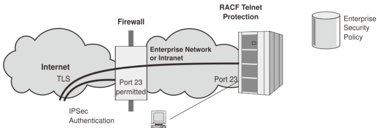
Figure 36. Secure and non-secure traffic using a single Telnet port
