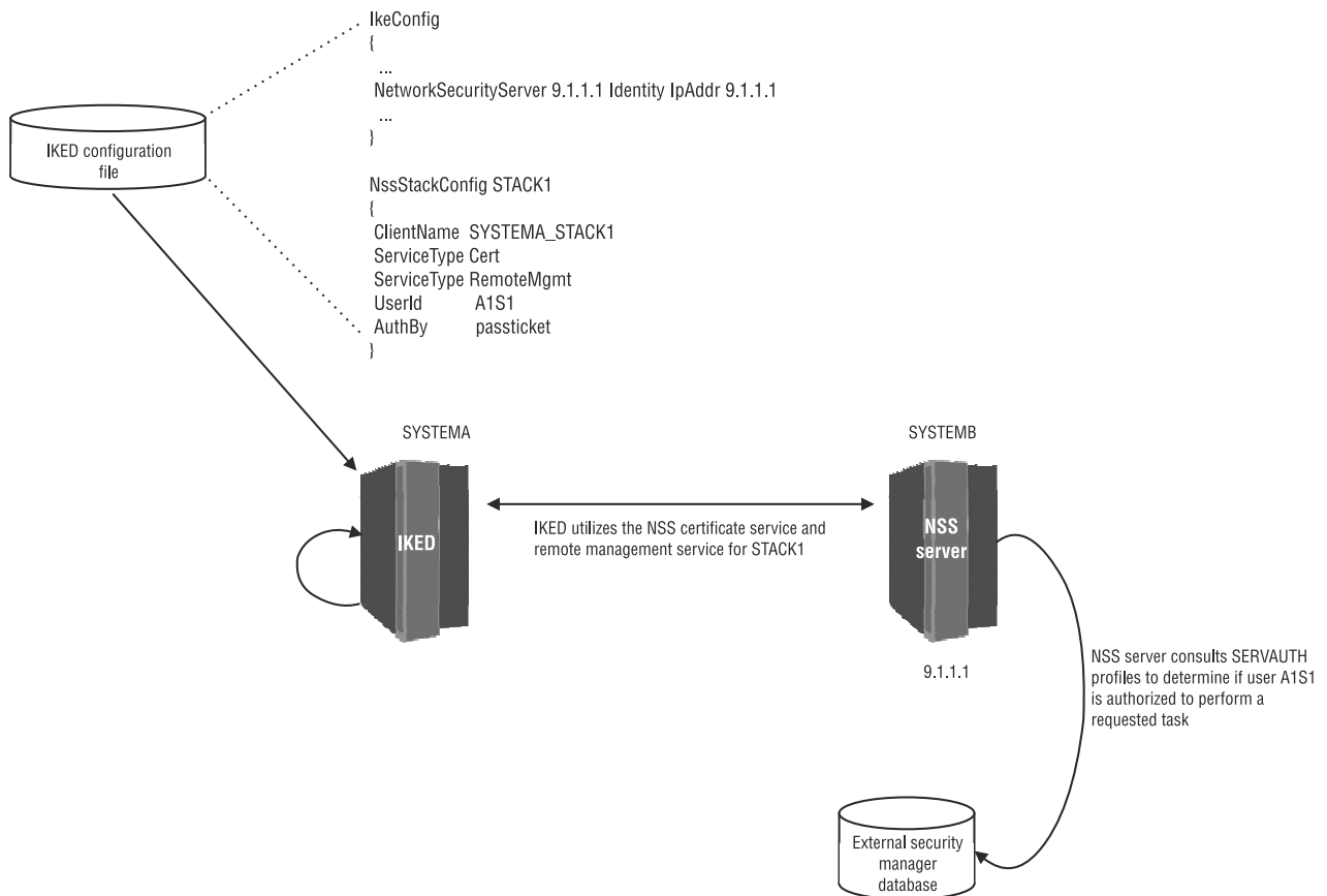
Figure 131. Enabling network security services
