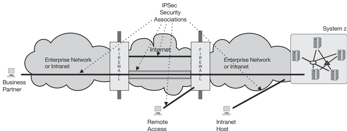
Figure 32. e-business scenarios with virtual private networks
