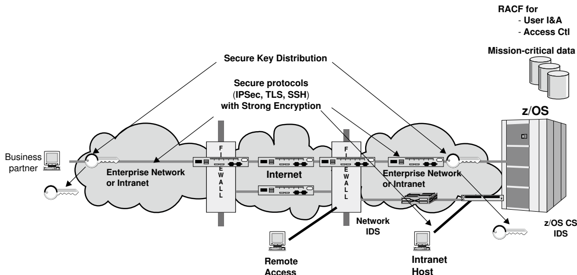
Figure 26. Elements of a secure TCP/IP deployment
