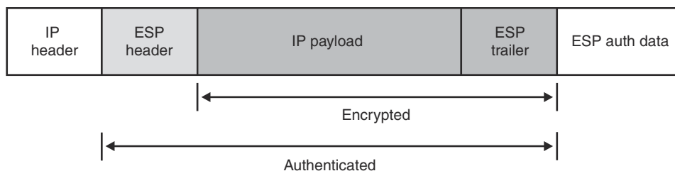
Figure 108. IPv4 packet encapsulated using ESP in transport mode
