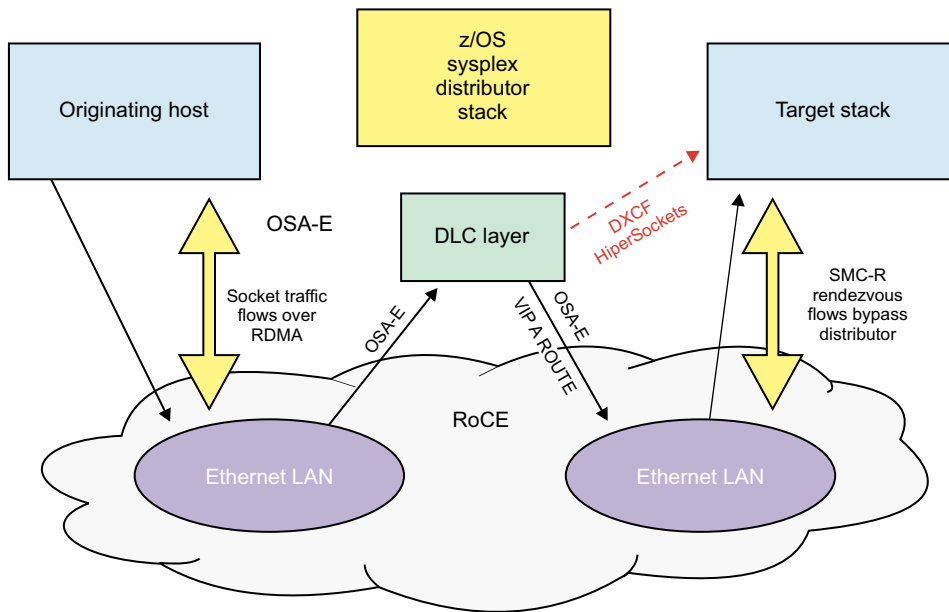
Figure 79. Sysplex distributor and SMC-R interaction
