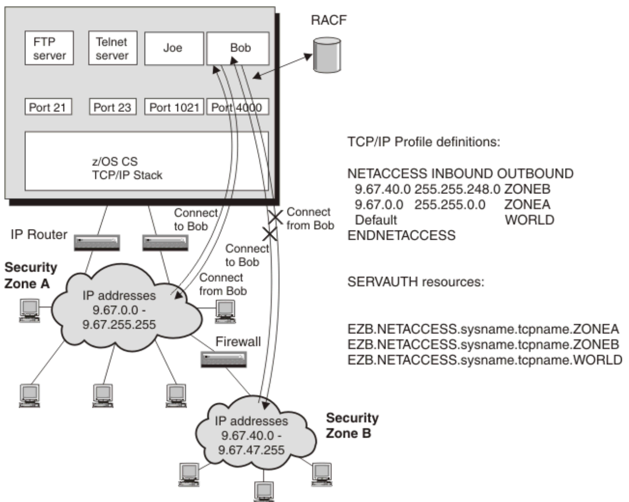
Figure 29. Network access control example
