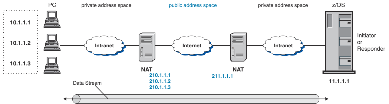
Figure 129. z/OS host to non-z/OS host, double NAT
