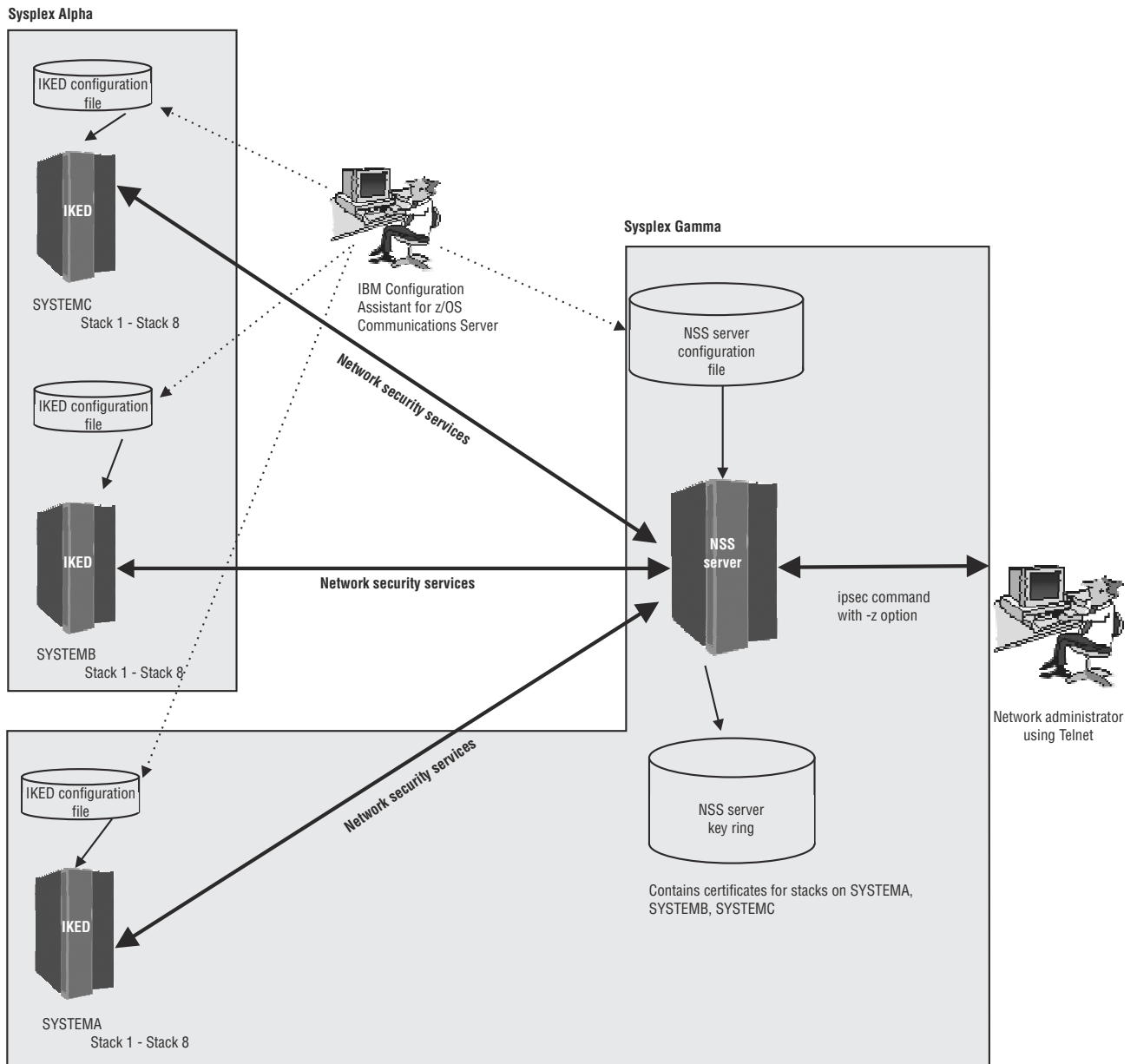
Figure 43. IKE daemon acting as an NSS client for multiple TCP/IP stacks
