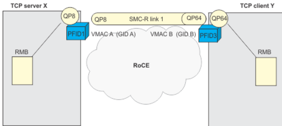
Figure 78. SMC-R link group with no redundant link
