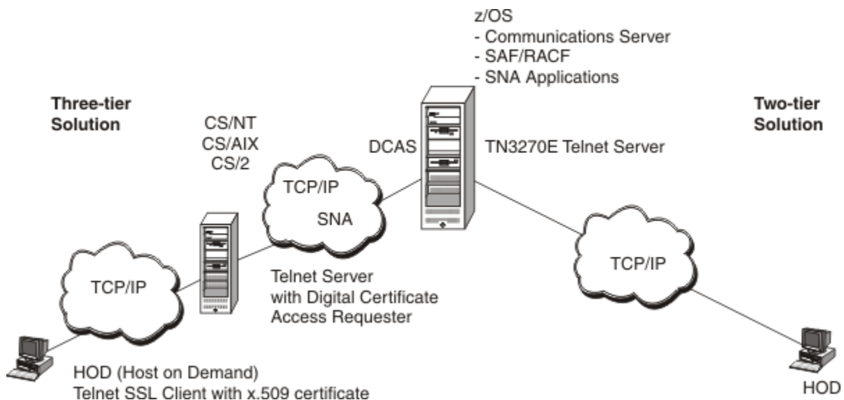
Figure 156. Express Logon network
