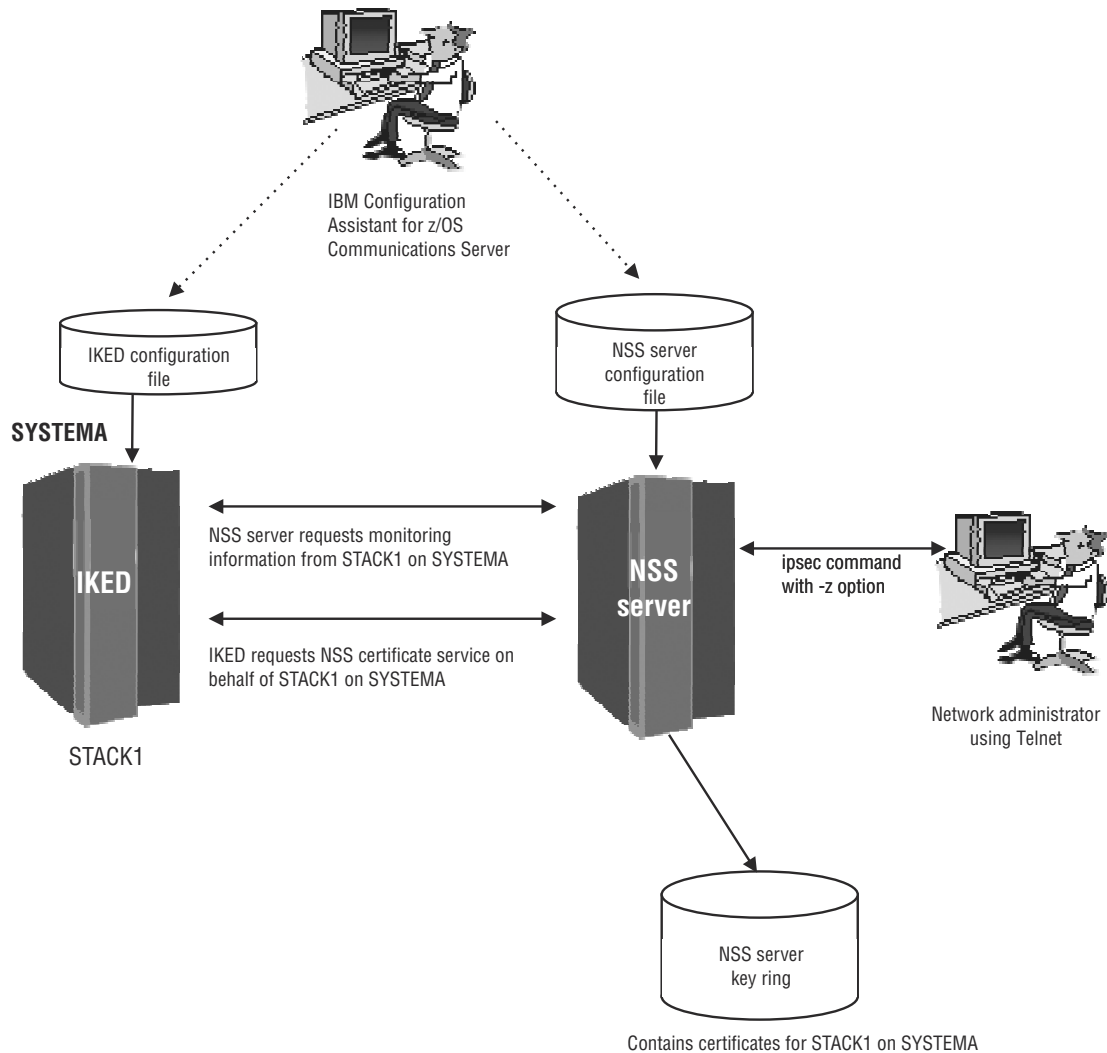
Figure 42. IKE daemon acting as an NSS client for a single TCP/IP stack
