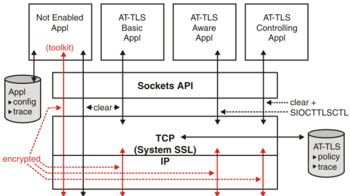
Figure 135. Application Transparent TLS
