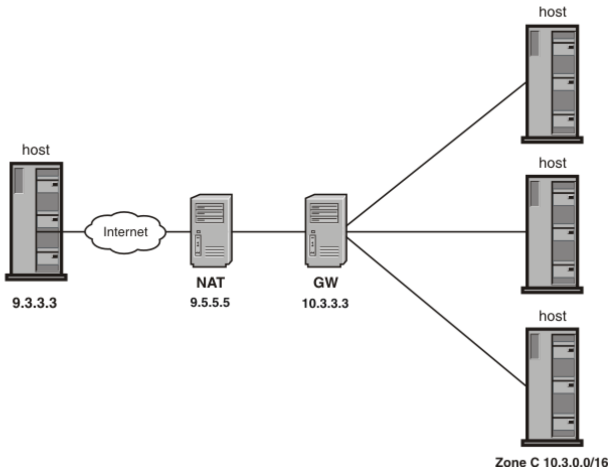
Figure 125. Branch office with NAT model
