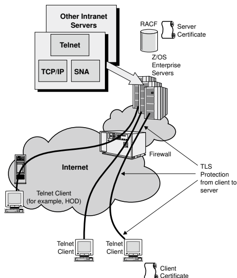
Figure 33. TN3270E Telnet server security overview
