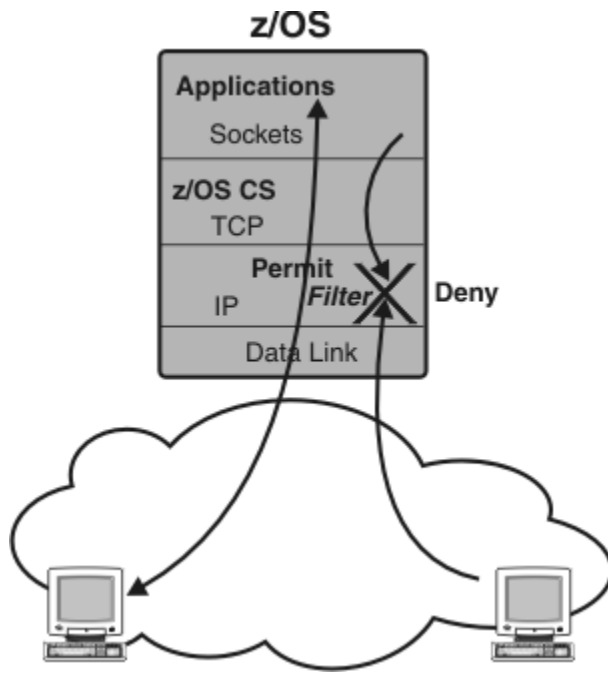
Figure 30. IP filtering at the z/OS communication endpoint
