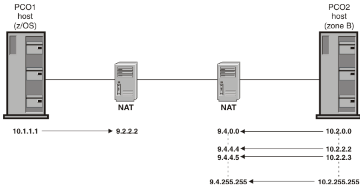
Figure 122. Partner company with NAT model
